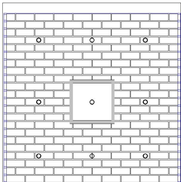
Figure 4; Spray Nozzle Locations
