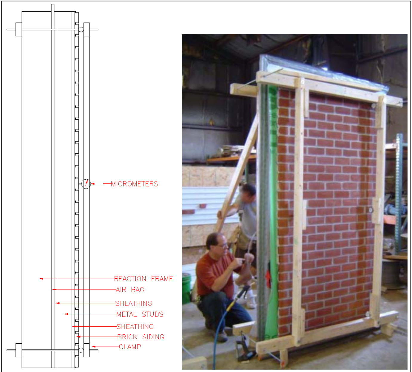
Figure 6; E72 Flexural Test
