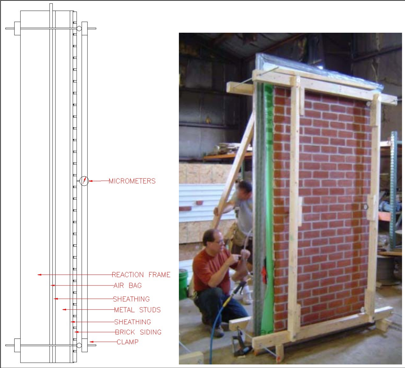
Figure 6; E72 Flexural Test
